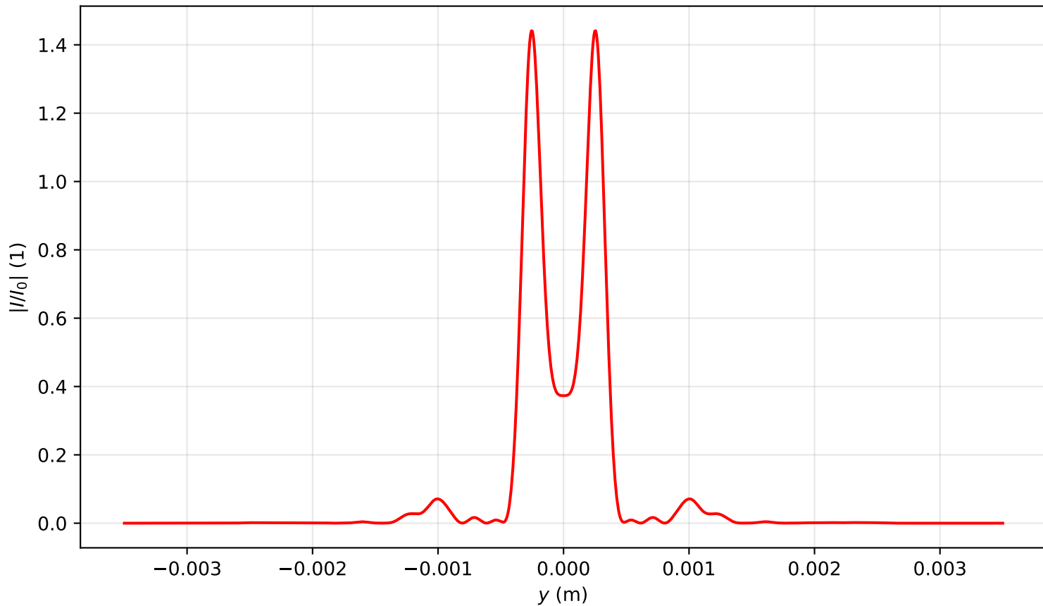
Intensity profile I(x=0, y, z=1.433)/I_0 , P_{in}=4.5P_{cr} , artificial time
